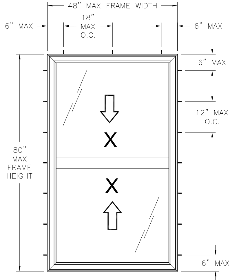
CAMBRIDGE DOUBLE HUNG EXTERIOR VIEW FRAME INSTALLATION
