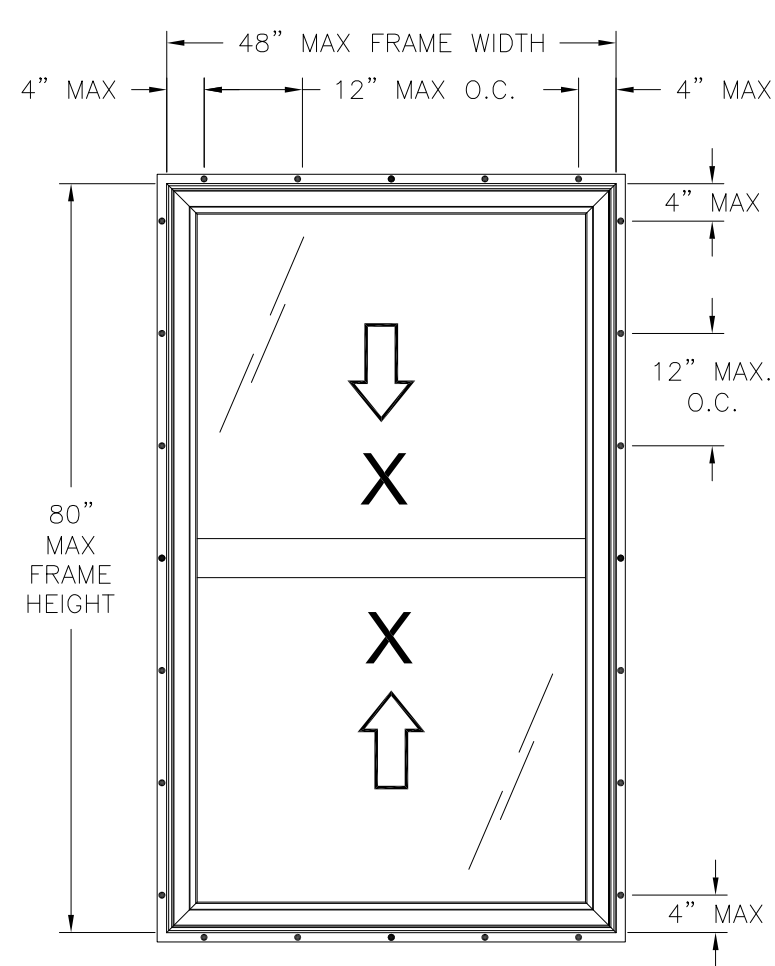
S-SERIES DOUBLE HUNG EXTERIOR VIEW FIN INSTALLATION
